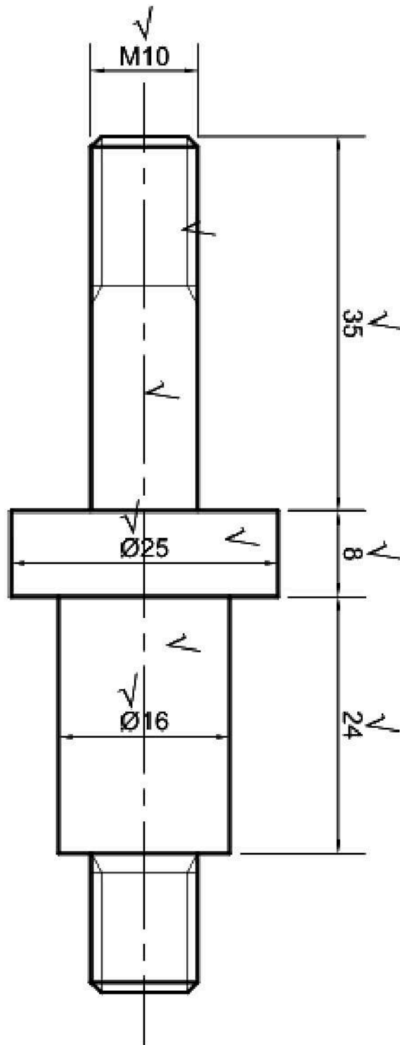
THE DRIVING PIN (ITEM 2)
