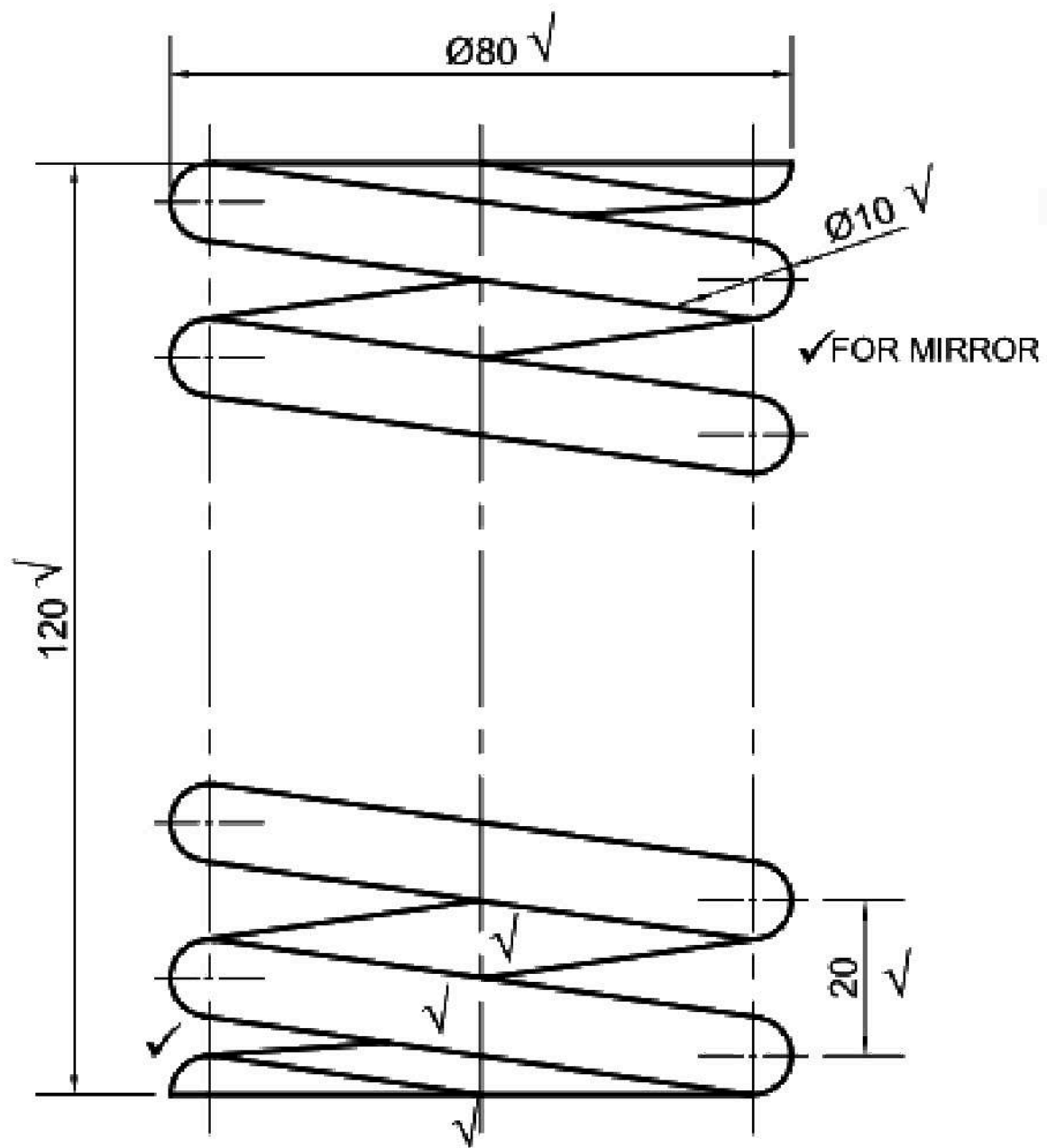
HELICAL SPRING ✓ SCALE 1:1 ✓
