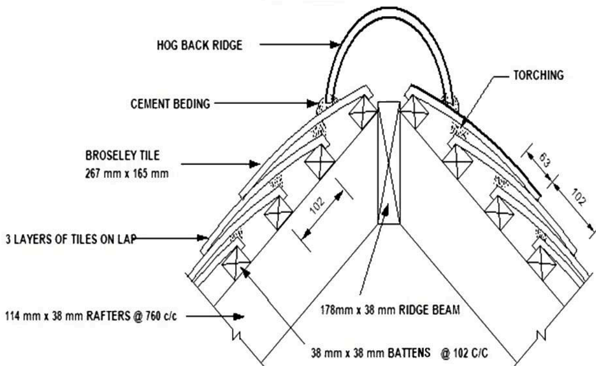
VERTICAL SECTION THROUGH THE RIDGE SCALE 1:5
