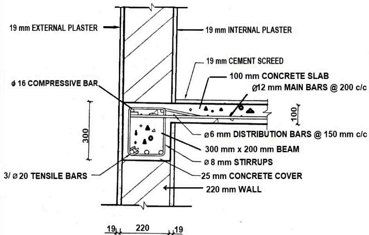
REINFORCEMENT CONCRETE BEAM SCALE 1:10
