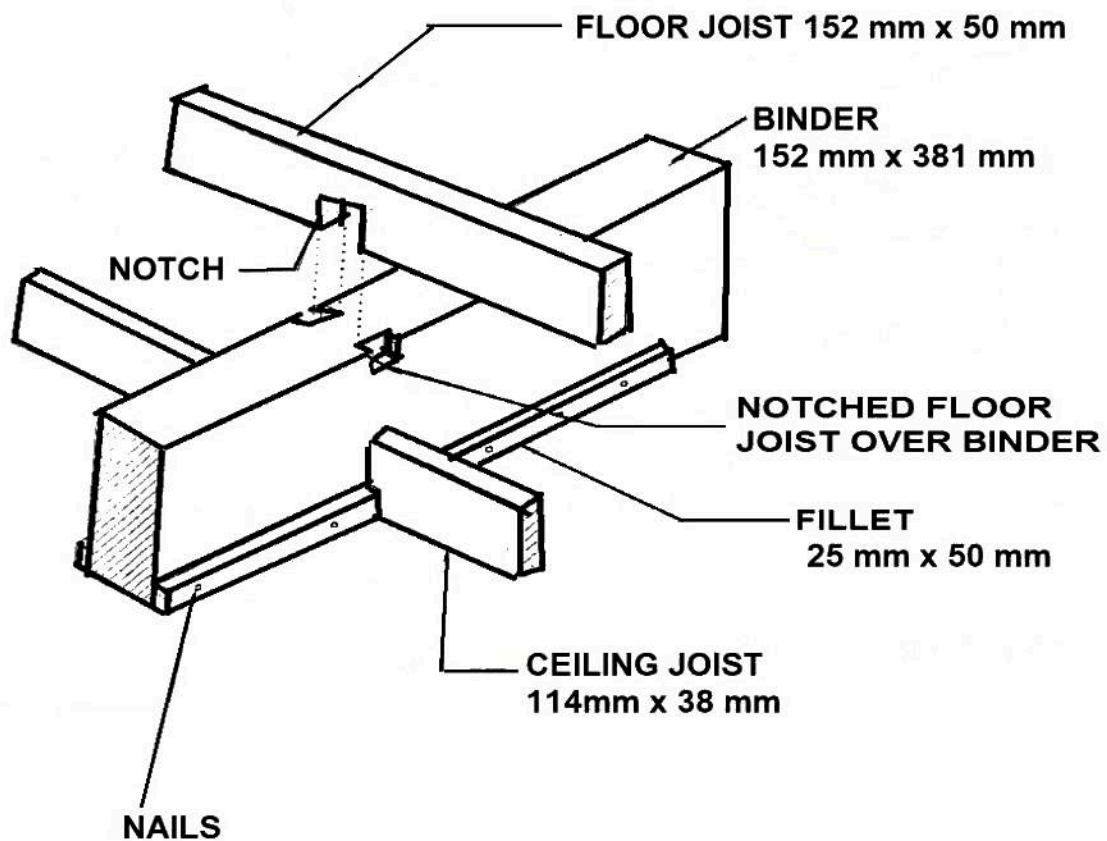
ISOMETRIC VIEW OF NOTCHED OR COGGED JOINT BETWEEN JOIST AND BINDER SCALE 1:5
