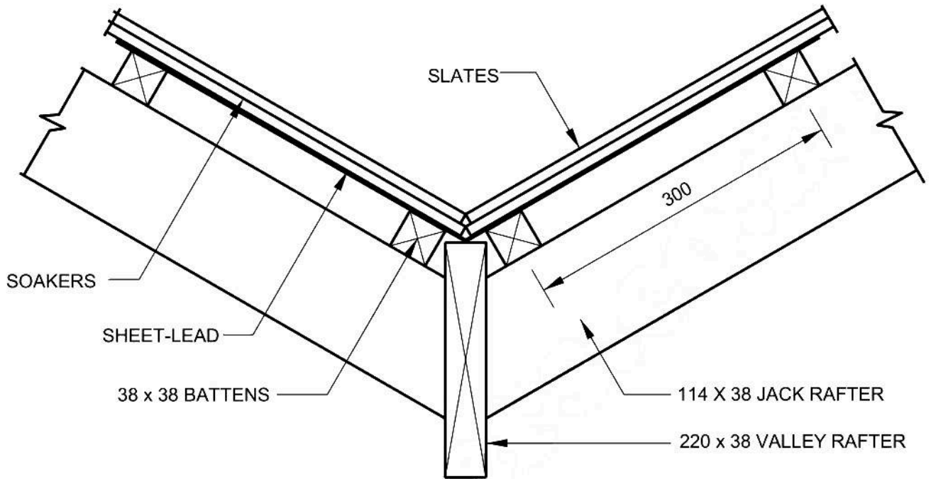
SECTION THROUGH CLOSED VALLEY
