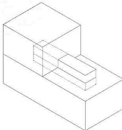
TABLING JOINT WITH SLATE JOGGLE
