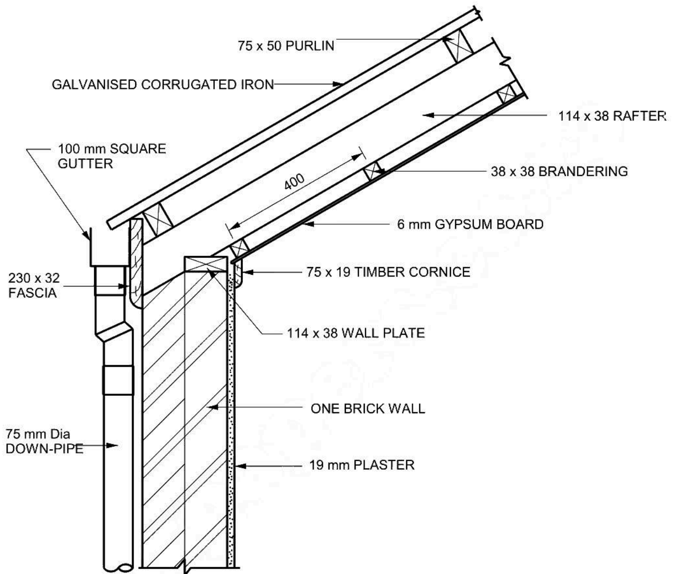
VERTICAL SECTION THROUGH FLUSH EAVES
