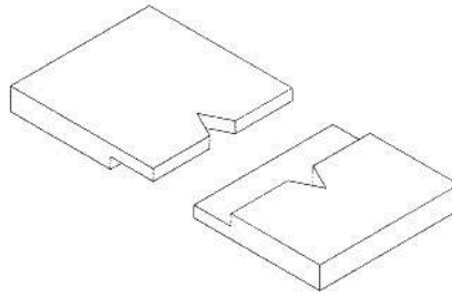
REBATED JOINT WITH JOGGLE
