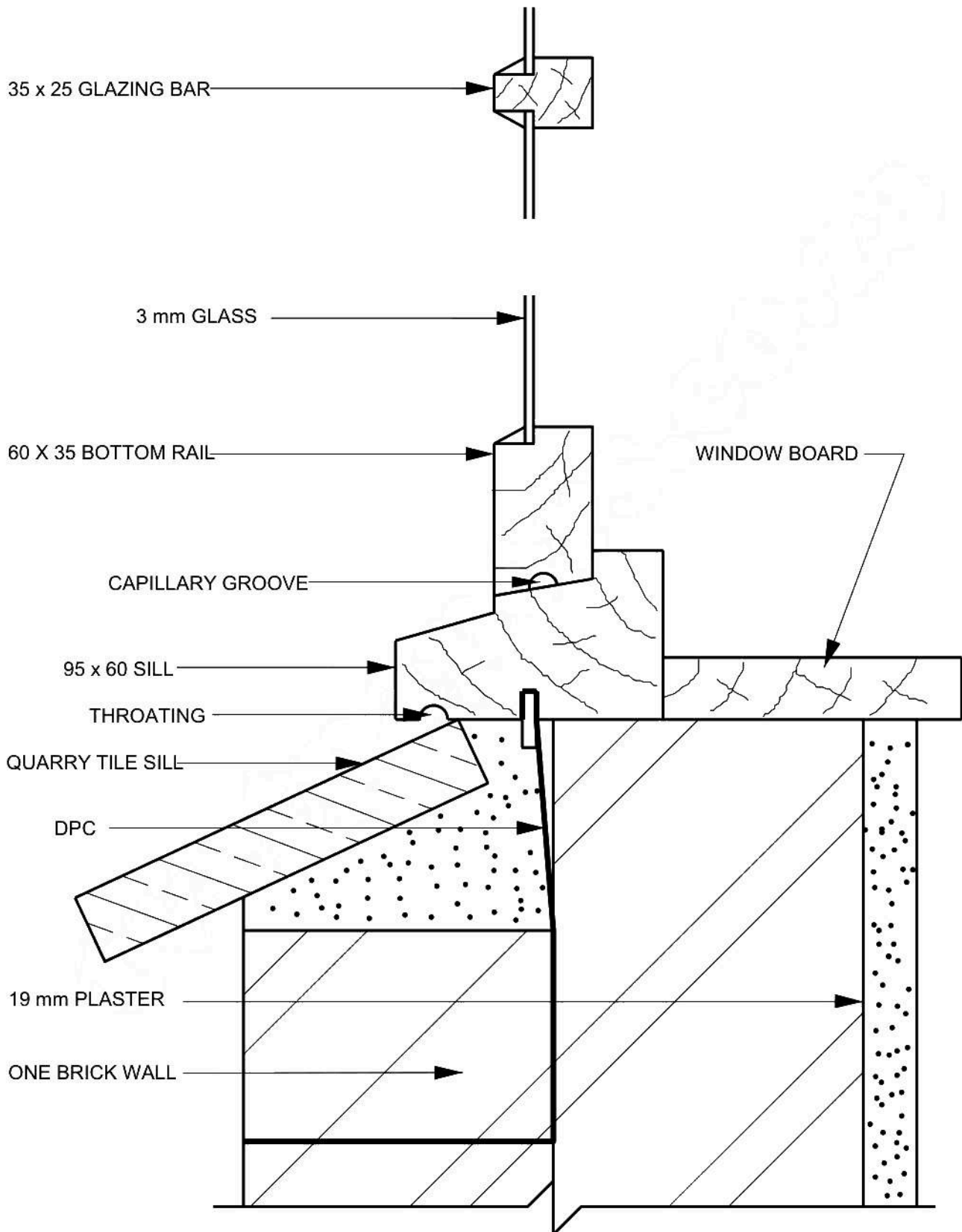
VERTICAL SECTION THROUGH GLAZING BAR AND WINDOW SILL
