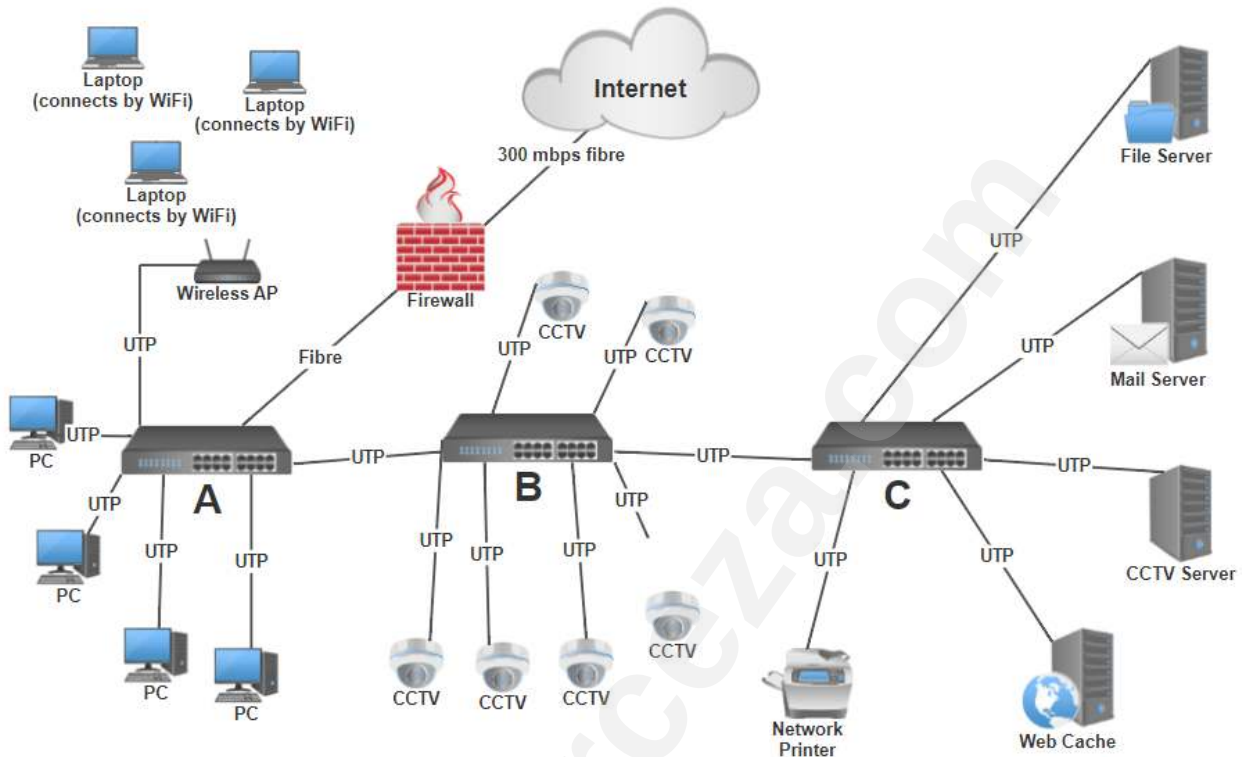
Network Layout
