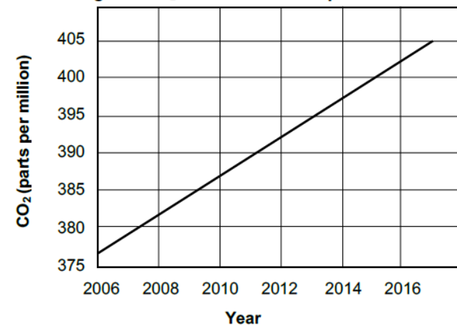
Changes in CO 2 levels in the atmosphere from 2006 to 2017
