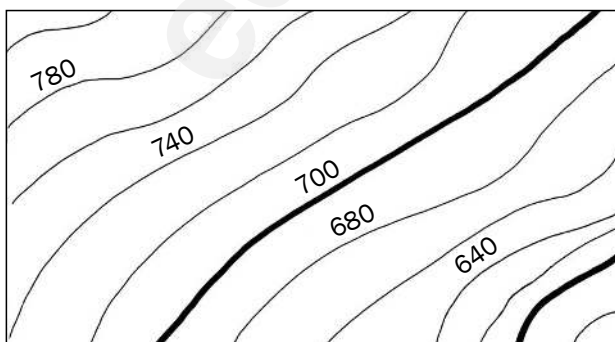
Figure 5.2.3: Countour lines of a steep slope
