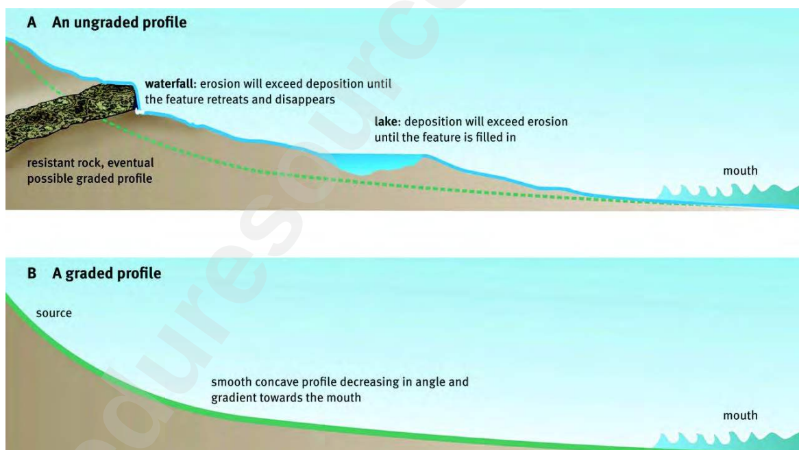
Figure 49 Comparison of a river with an ungraded profile (A) and a graded profile (B)
