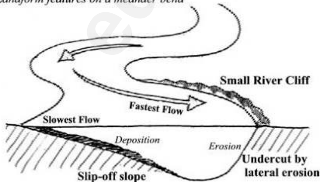
Landform features on a meander bend
