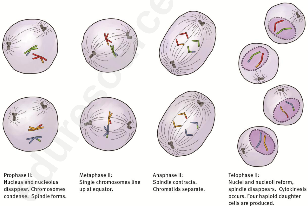
Figure 7 Meiosis II
