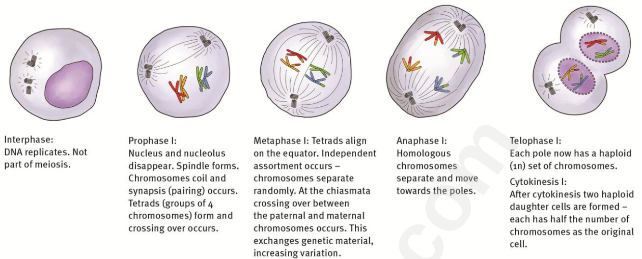
Figure 6 Meiosis I
