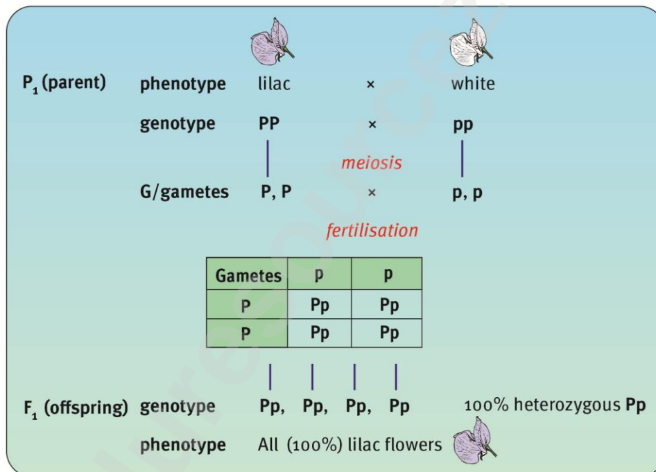
Figure 20 Monohybrid cross
