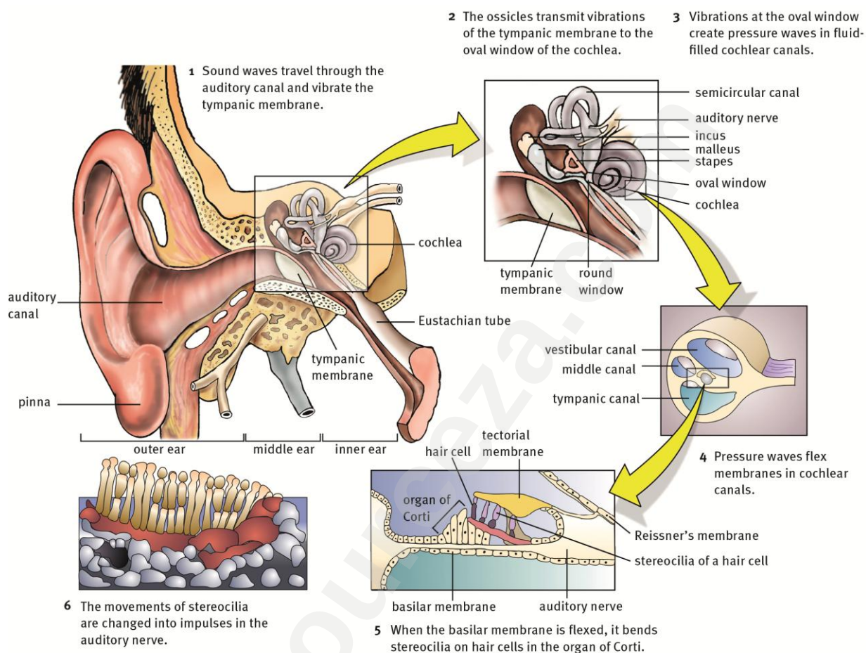
Figure 31 Hearing
