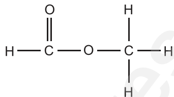
methyl methanoate
