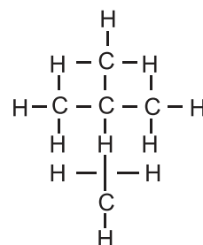
2,2-dimethylpropane
