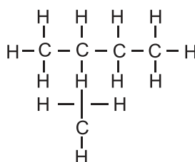
2-Methylbutane
