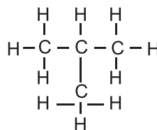
2-methylpropane
