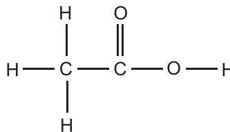
ethanoic acid
