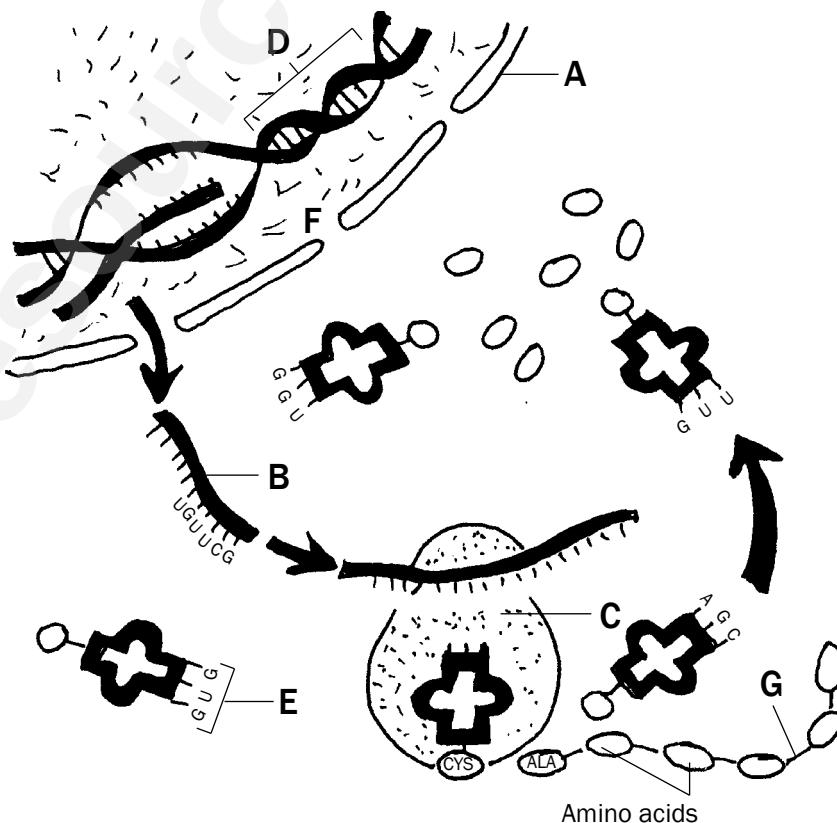
Figure 1.7 Protein synthesis
