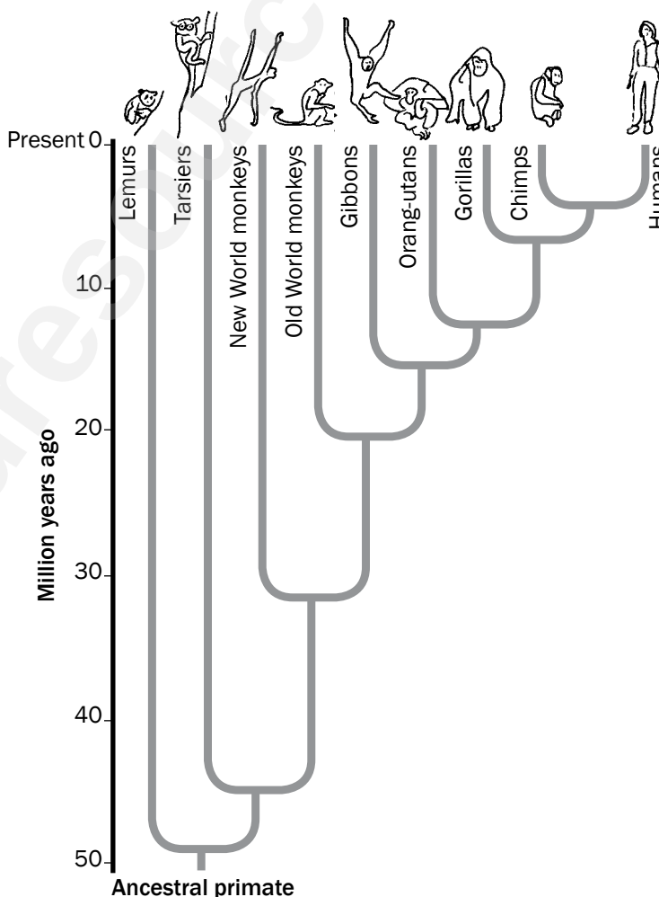
Figure 10.11 Phylogenetic tree
