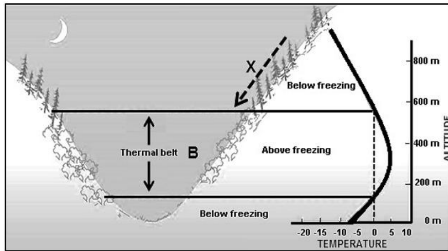
FIGURE 1.4: VALLEY CLIMATES
