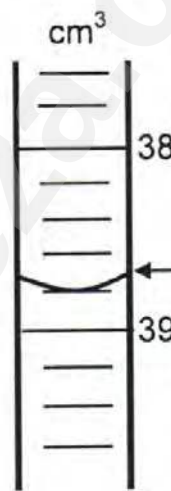
At the endpoint
