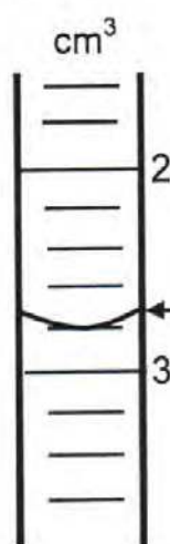
Before the titration
