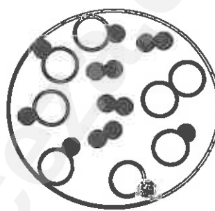
Reaction mixture at equilibrium
