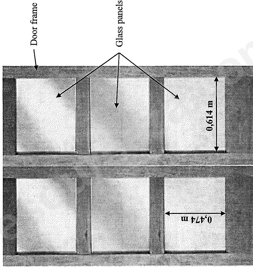
PICTURE OF THE ENTRANCE DOOR WITH INNER DIMENSIONS OF THE ORIGINAL GLASS PANELS
