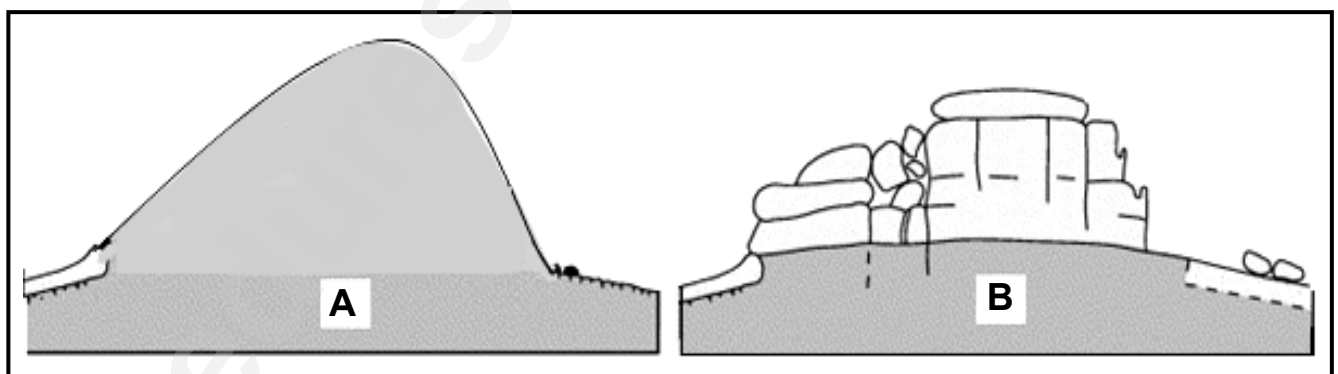
FIGURE 1.6: LANDFORMS ASSOCIATED WITH VOLCANIC ACTIVITY
