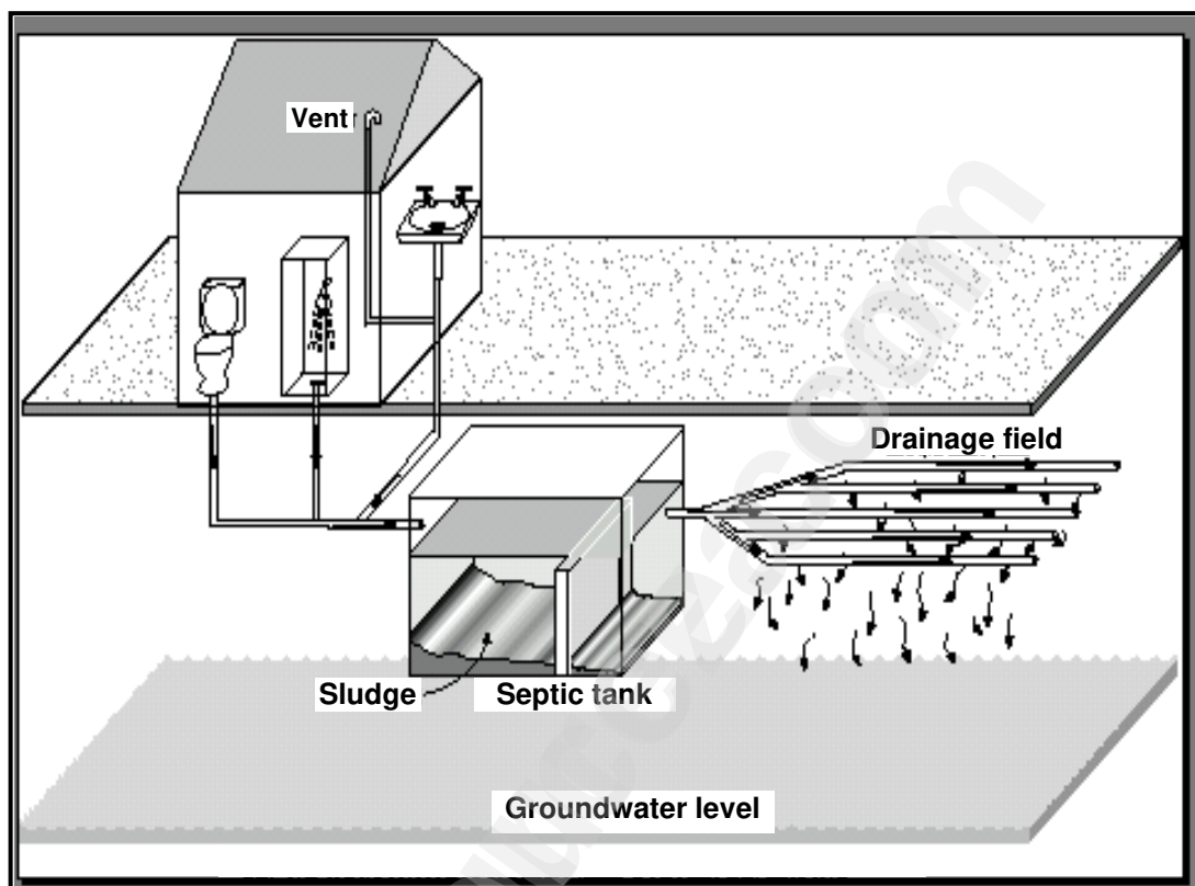
Septic tank with drainage field system
