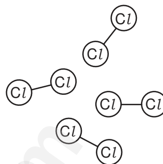
chlorine
